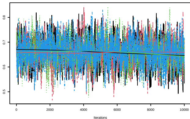
Trace of lambda.y.strd[2]
