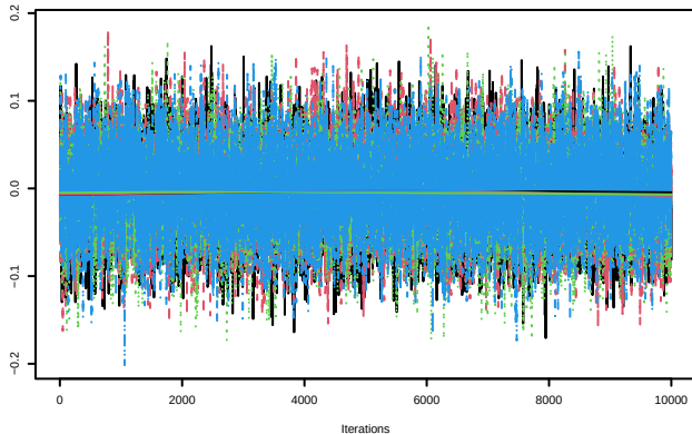
Trace of sigma.eps[1]
