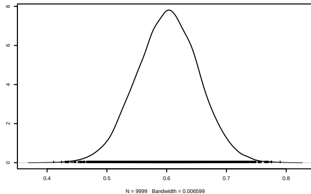
Density of \lambda_{\text{bda.y}[1]}
