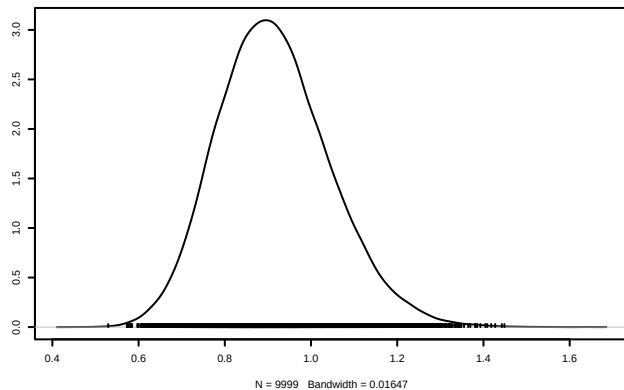
Density of \lambda_{\text{bda.y}[2]}
