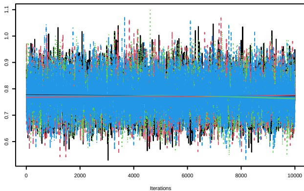
Trace of sigma.eps[3]
