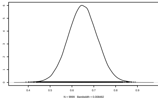
Density of sigma.eta
