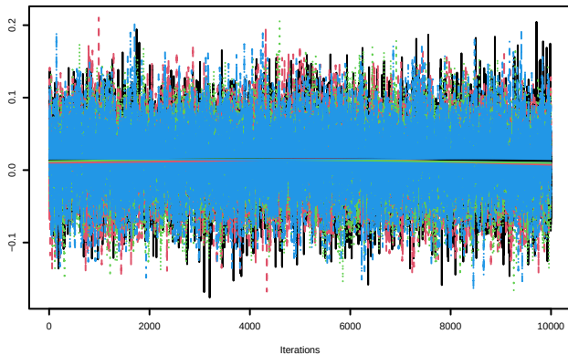
Trace of nu.y[2]
