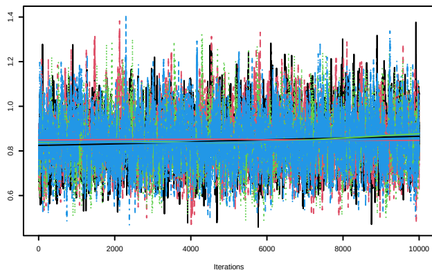
Trace of \lambda_{\text{bda.y}[2]}
