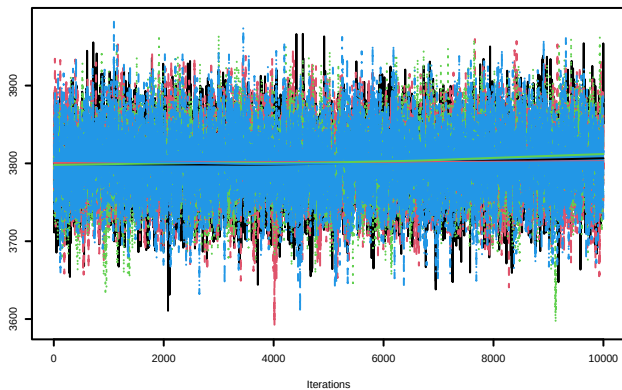
Trace of lambda.y.strd[1]
