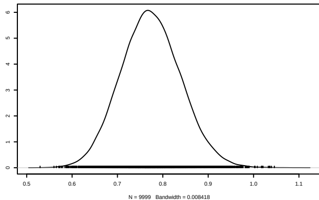
Density of sigma.eps[3]
