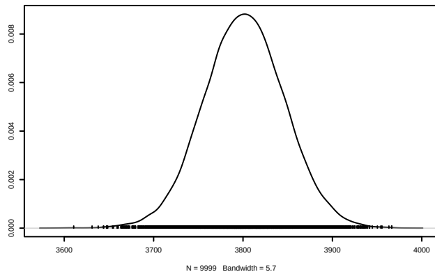
Density of lambda.y.strd[1]
