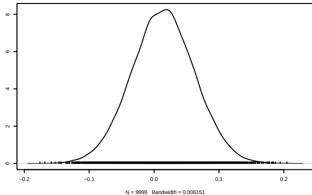
Density of nu.y[2]
