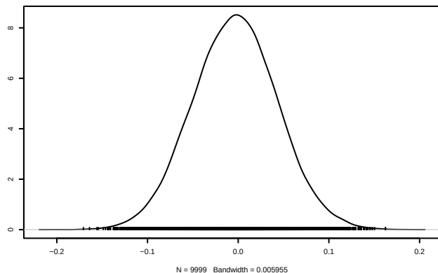
Density of sigma.eps[1]
