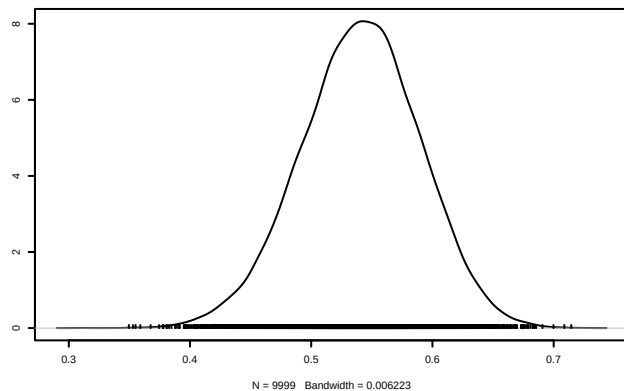
Density of lambda.y.strd[2]
