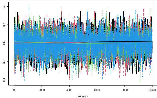
Trace of \lambda_{\text{bda.y}[1]}
