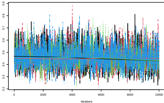
Trace of sigma.eta
